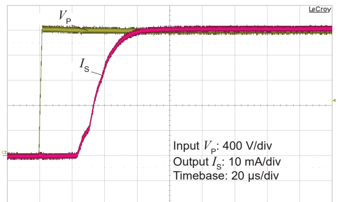
Figure 6: Typical step response (0 to 2000 V)
