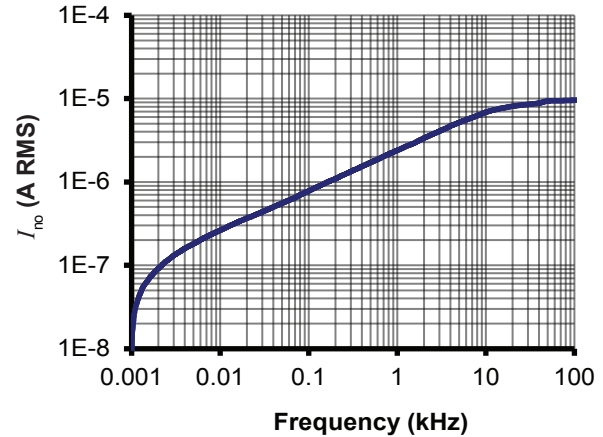
Figure 14: Typical total output RMS noise current with R_M = 50 \Omega
