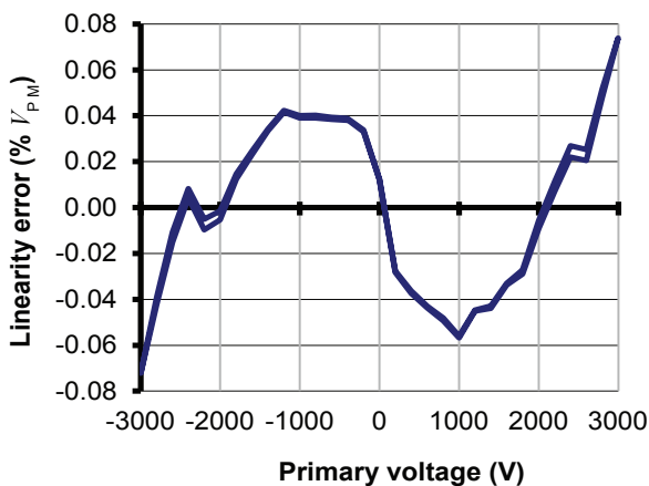
Figure 15: Typical linearity error at 25 °C
