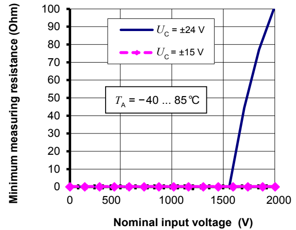
Figure 2: Minimum measuring resistance
